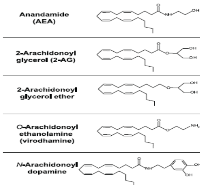
Figure 2. Chemical structure of endogenous cannabinoid
