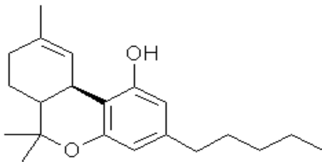
Figure 1. Chemical structure of \Delta^9 -tetrahydrocannabinol
